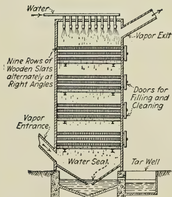
FIG. 63.—Hurdle Scrubber Filled with Wooden Slats.
